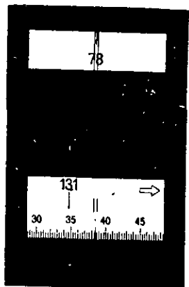
360° Limbo vertical 78° 38' 30"
