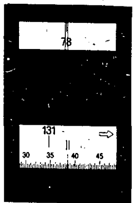
360° Limbo vertical 78° 38' 30"
