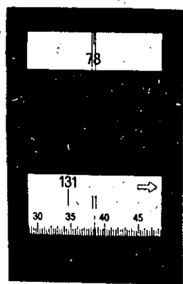
360° Limbo vertical 78° 38' 30"
