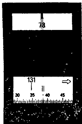
360° Limbo vertical 78° 38' 30"
